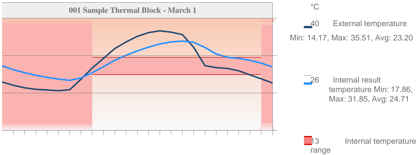
Figure 28: Energy evaluation of University of Lagos Women Society Hall.
